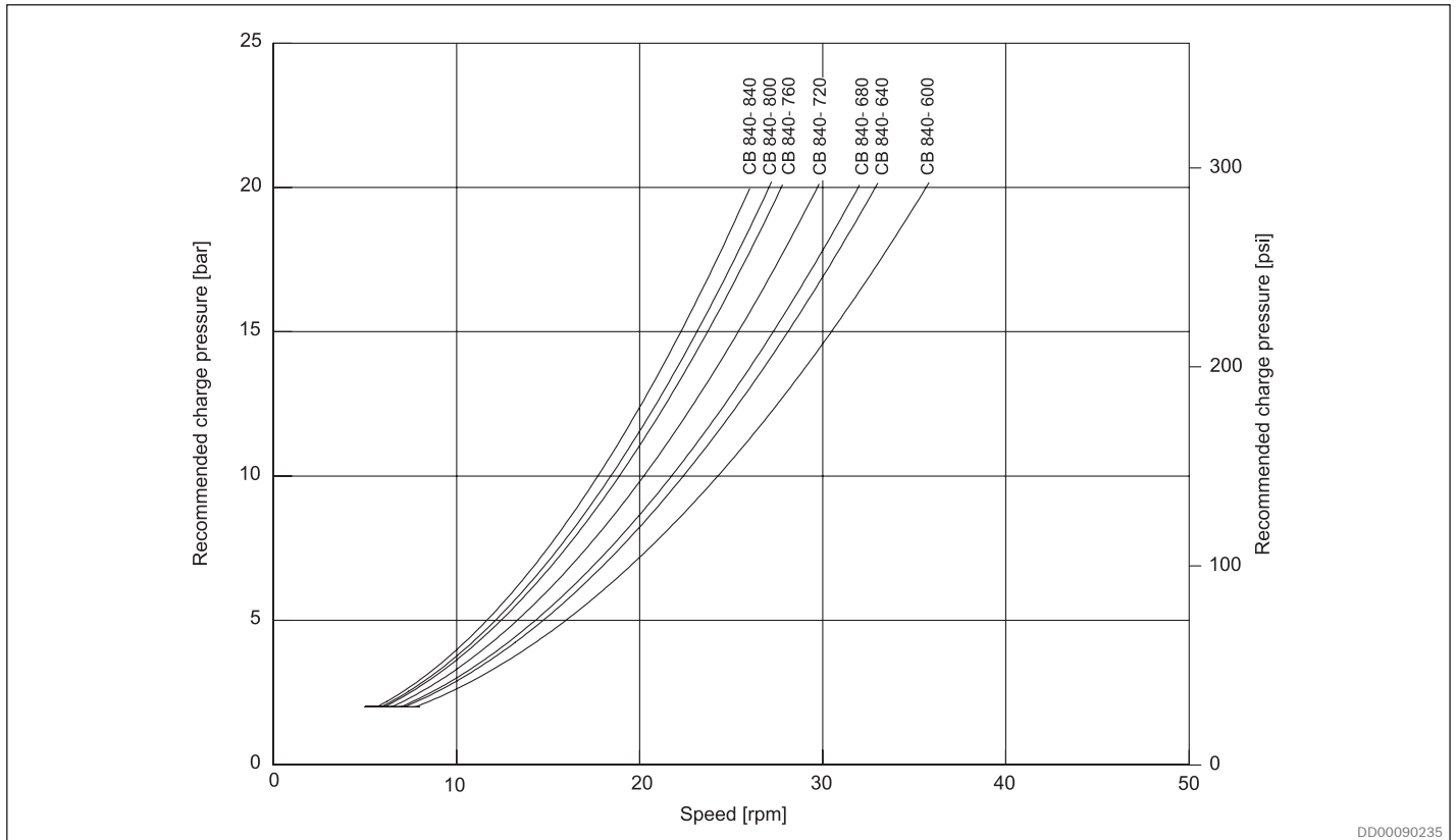
Fig. 9: Recommended charge pressure for motor working in braking mode, Hägglands CB 840, 2-port connection. Valid for oil viscosity 40 cSt.
