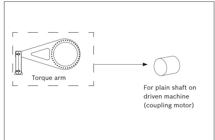
Fig. 85: Single ended torque arm mounting for plain shaft
