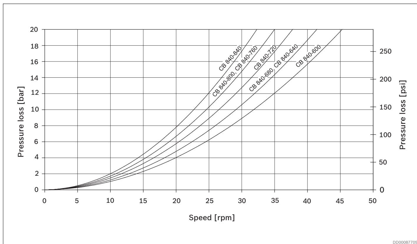
Fig. 46: CB 840 pressure loss 4 ports
