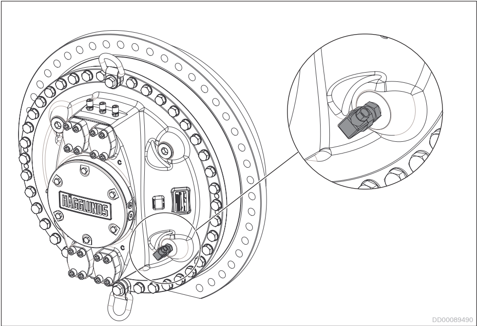
Fig. 92: Temperature sensor
