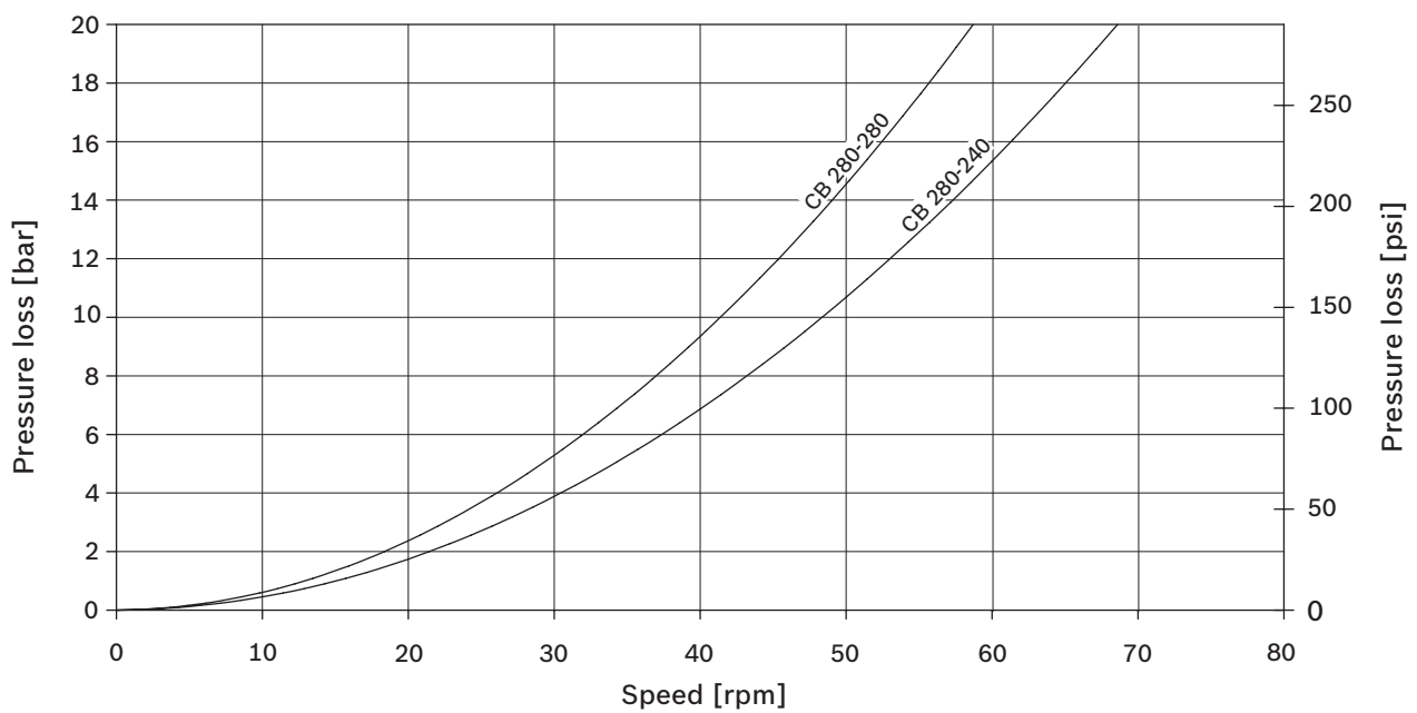
Fig. 40: CB 280 pressure loss 4 ports
