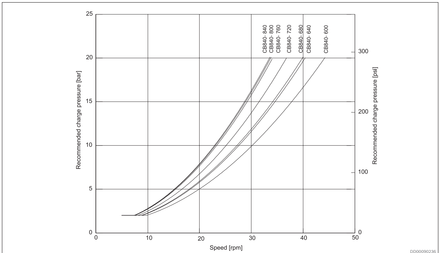
Fig. 10: Recommended charge pressure for motor working in braking mode, Hägglands CB 840, 4-port connection. Valid for oil viscosity 40 cSt.
