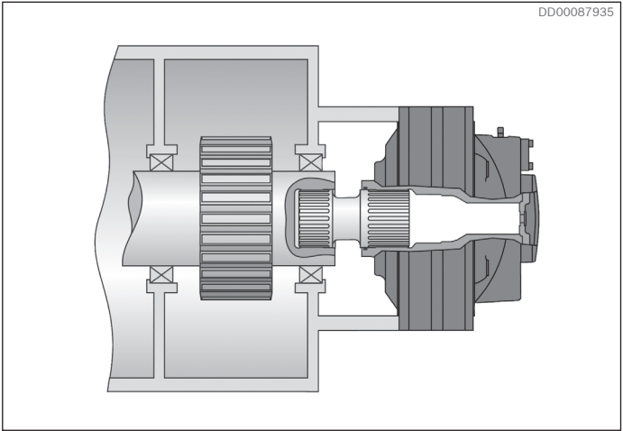
Fig. 78: Flange mounted motor with splines to avoid high radial load from driven shaft.
