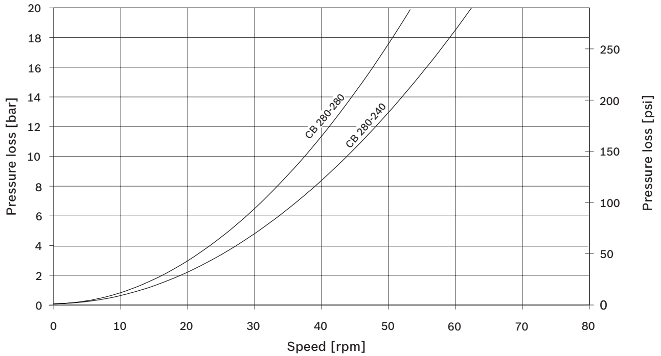
Fig. 39: CB 280 pressure loss 2 ports
