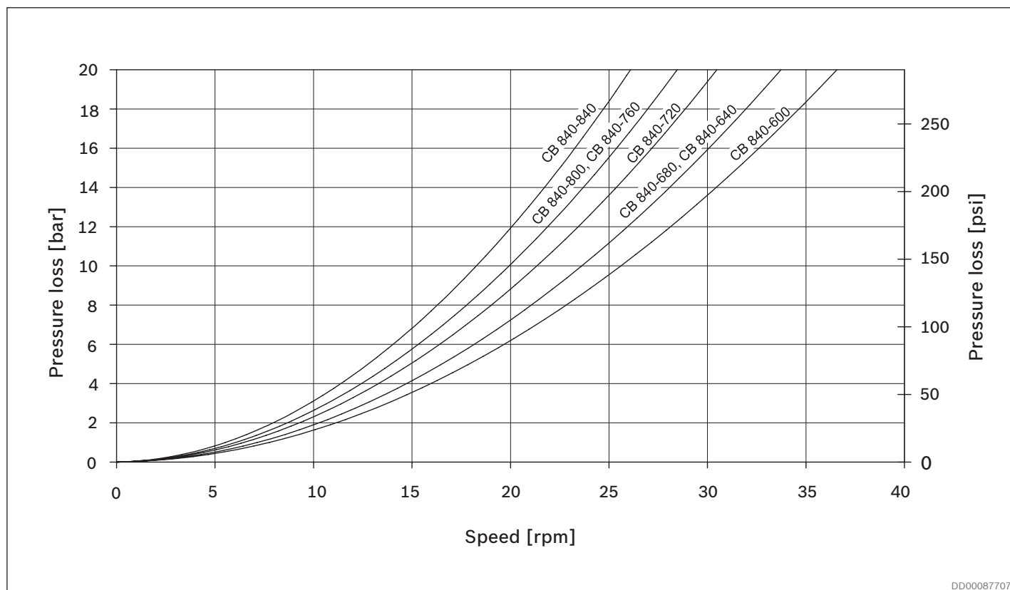
Fig. 45: CB 840 pressure loss 2 ports
